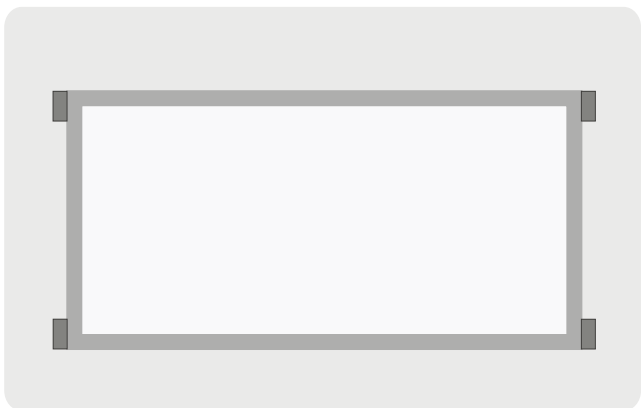
Clamps are mounted at the corners of short frame-Back side (clamp length \geq 60\text{mm} , the overlap of clamp and frame \geq 9\text{mm} )
