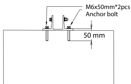
SOLID BLOCK SIDE VIEW
