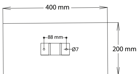
SOLID BLOCK TOP VIEW
